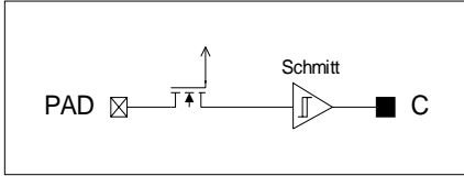
Figure 45 Digital Input with Schmitt Trigger
