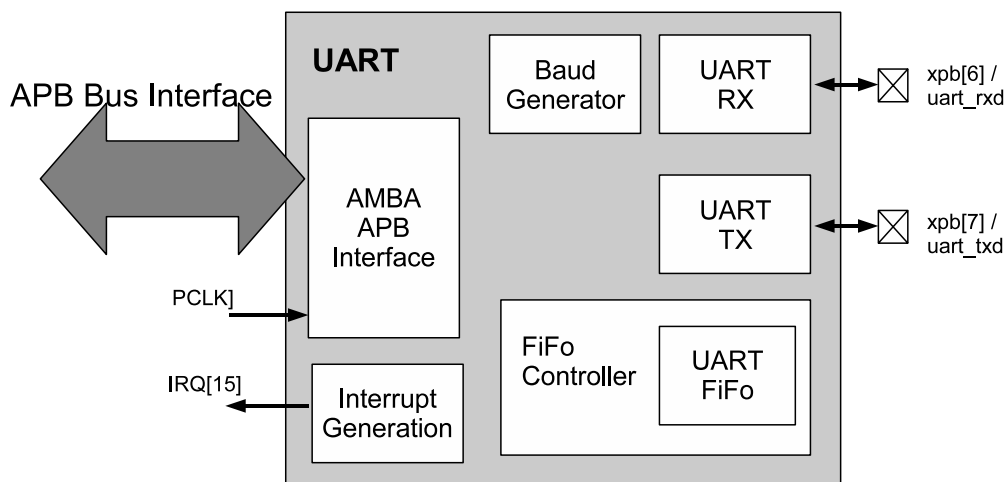
Figure 37 UART Block Diagram
