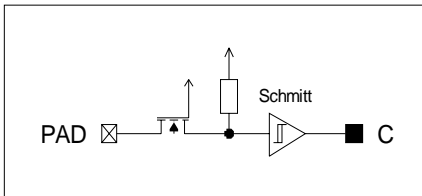
Figure 47 Digital Input with Schmitt Trigger and Pull-Up
