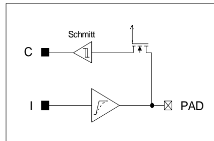
Figure 50 Digital Schmitt Trigger Input and Limited Slew Rate Output
