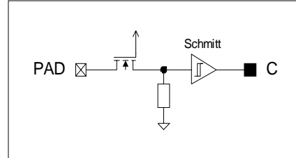
Figure 46 Digital Input with Schmitt Trigger and Pull-Down
