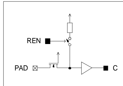
Figure 48 Digital Input with enable controlled Pull-Up
