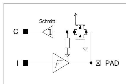
Figure 54 Digital Schmitt Trigger Input with Pull-Down and Limited Slew Rate Output (low voltage)
